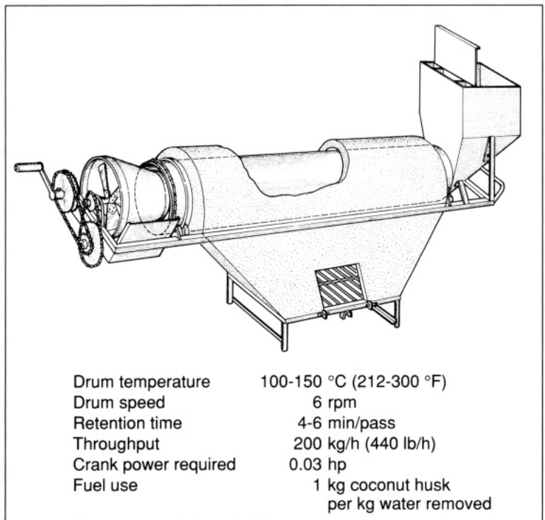
10.5. Conduction-type continuous-flow drum dryer.
