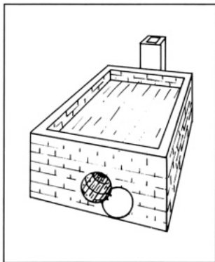
10.4. Oil-barrel dryer.
