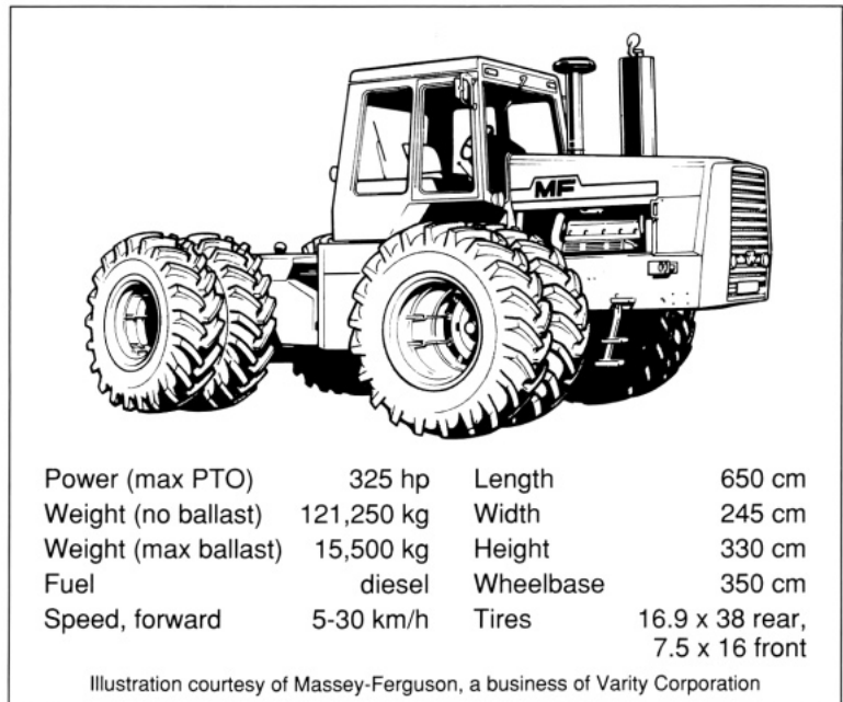
2.11. Four-wheel drive farm tractor.
