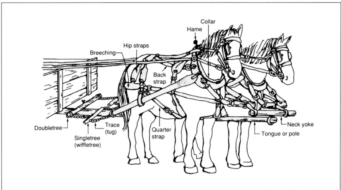
1.12. Harness for a team of two draft horses.
