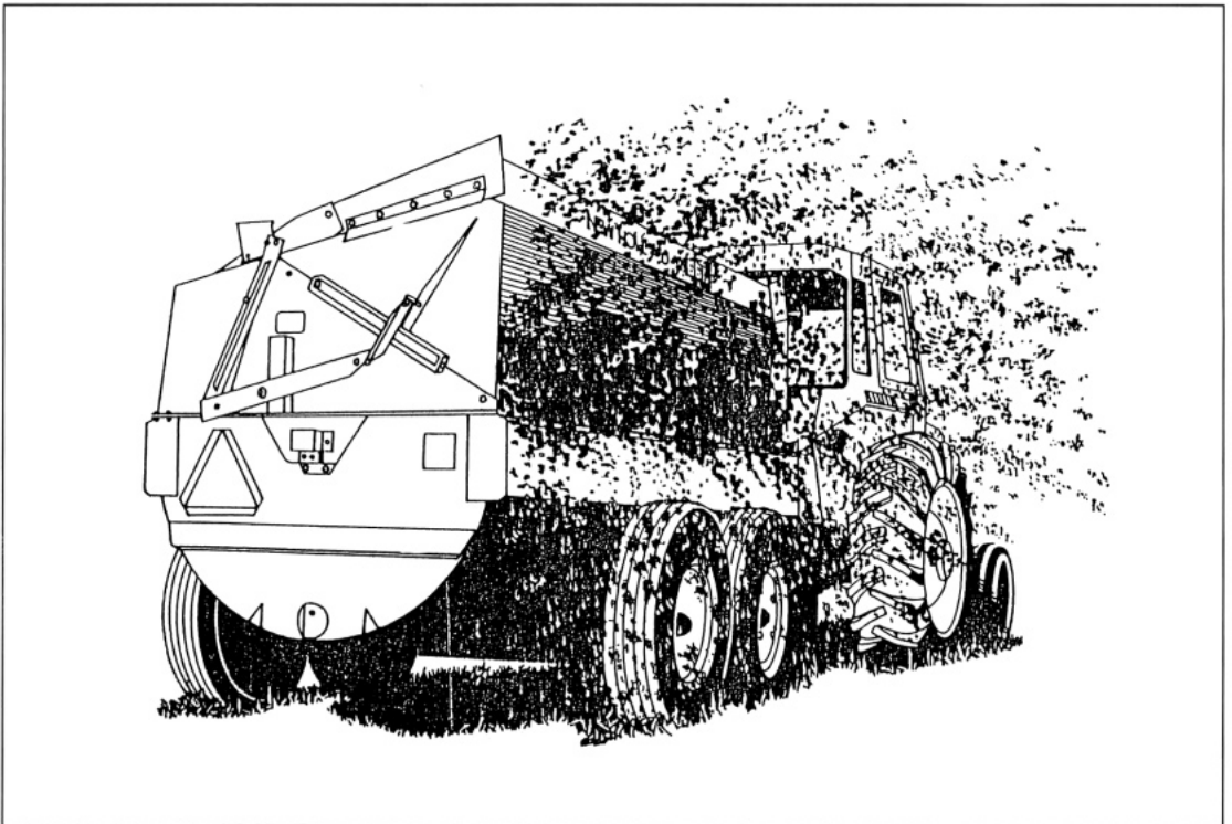
6.4. Flail-type manure spreader.
