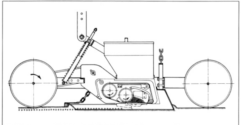
5.15. Single-seed planter with seed belt metering.
