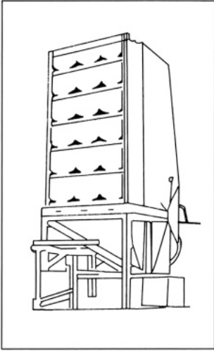
10.11. Mixing continuous-flow dryer.
