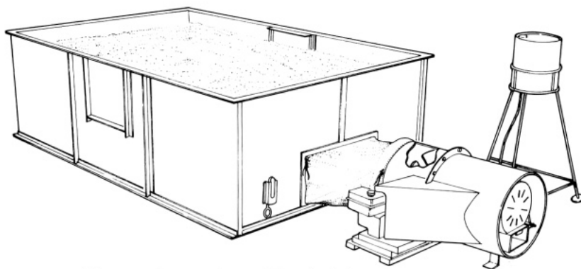
10.8. Flatbed dryer showing fan, burner, and bin.
