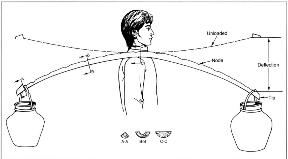
11.1. Bamboo carrying pole.
