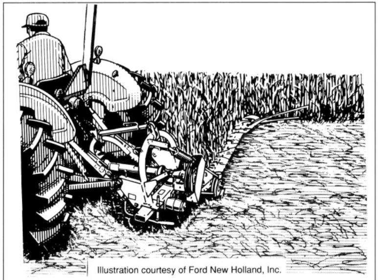
9.24. Reciprocating mower.
