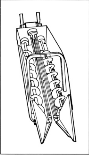
9.42. Stripping rolls of a cotton stripper.
