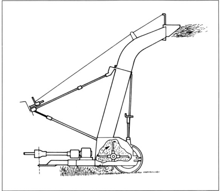
9.32. Flail forage harvester.
