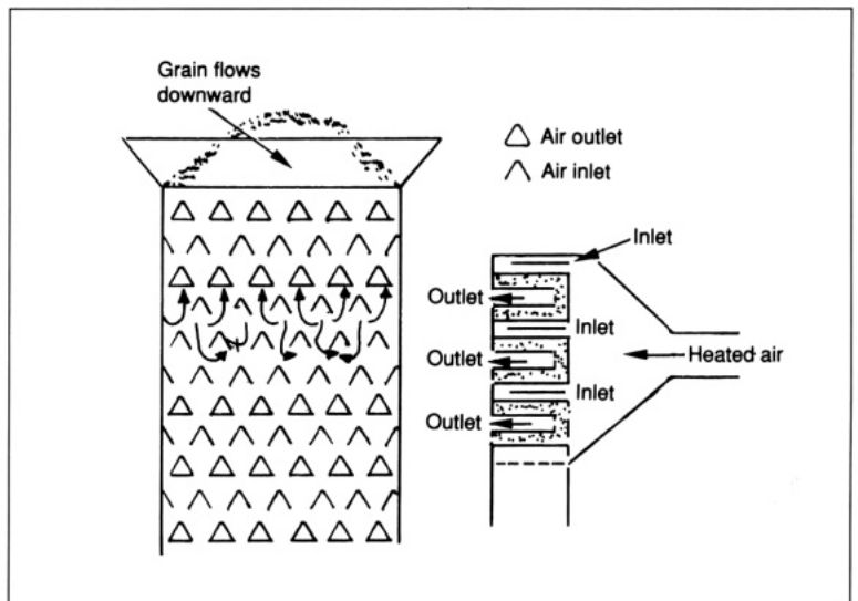
10.12. Flow pattern in the LSU mixing-type dryer.
