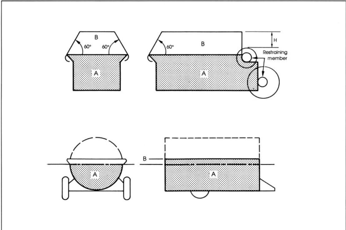
6.3. Volumetric capacity of box-type manure spreaders.
