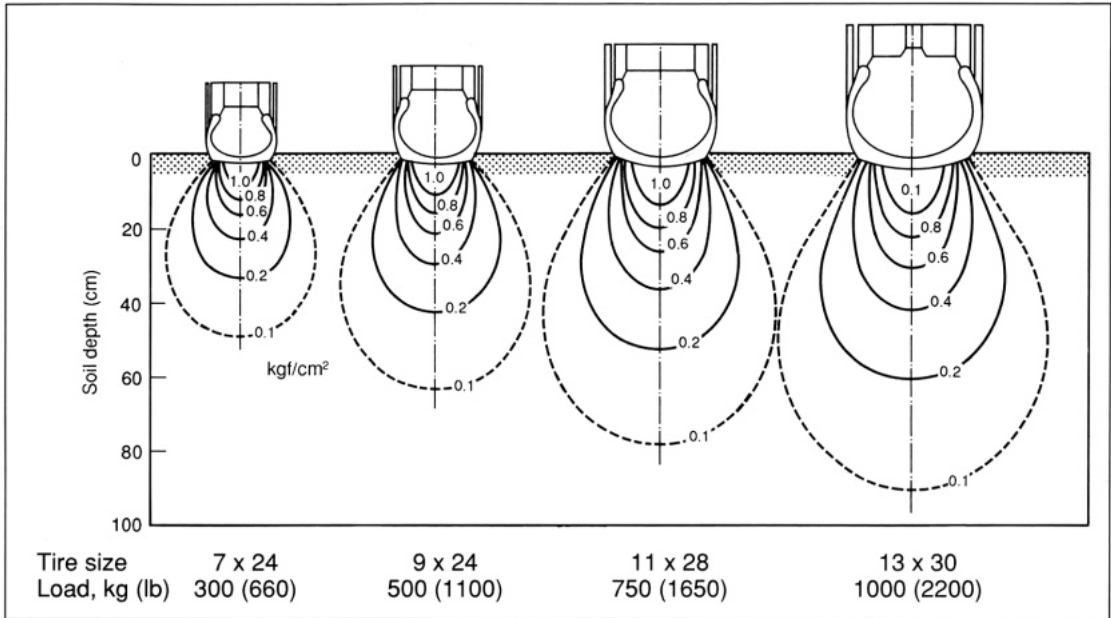
3.3. Isopressure lines under pneumatic tractor tire. 11
