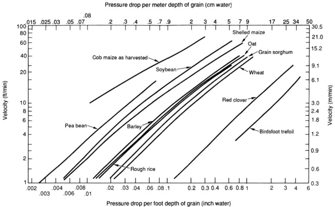
10.6. Shedd's Chart of resistance of grains to airflow.
