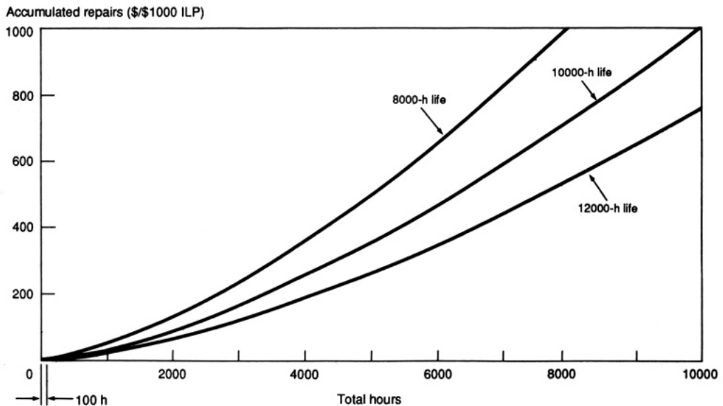
13.1. Accumulated cost of repairs for repair group 1.
