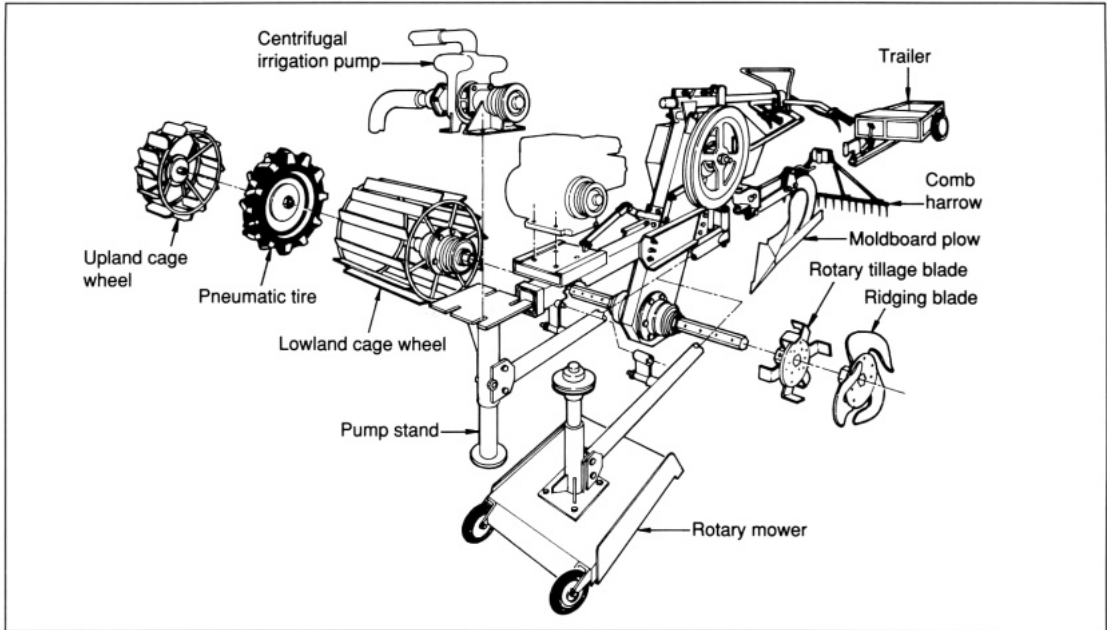
2.3. Single-axle pedestrian tractor and attachments.
