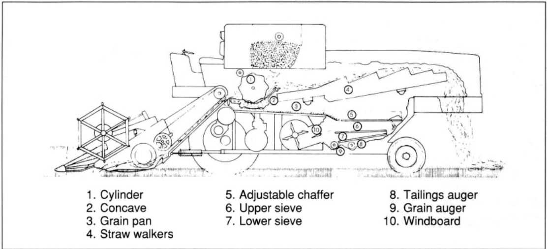
9.17. A conventional self-propelled combine.
