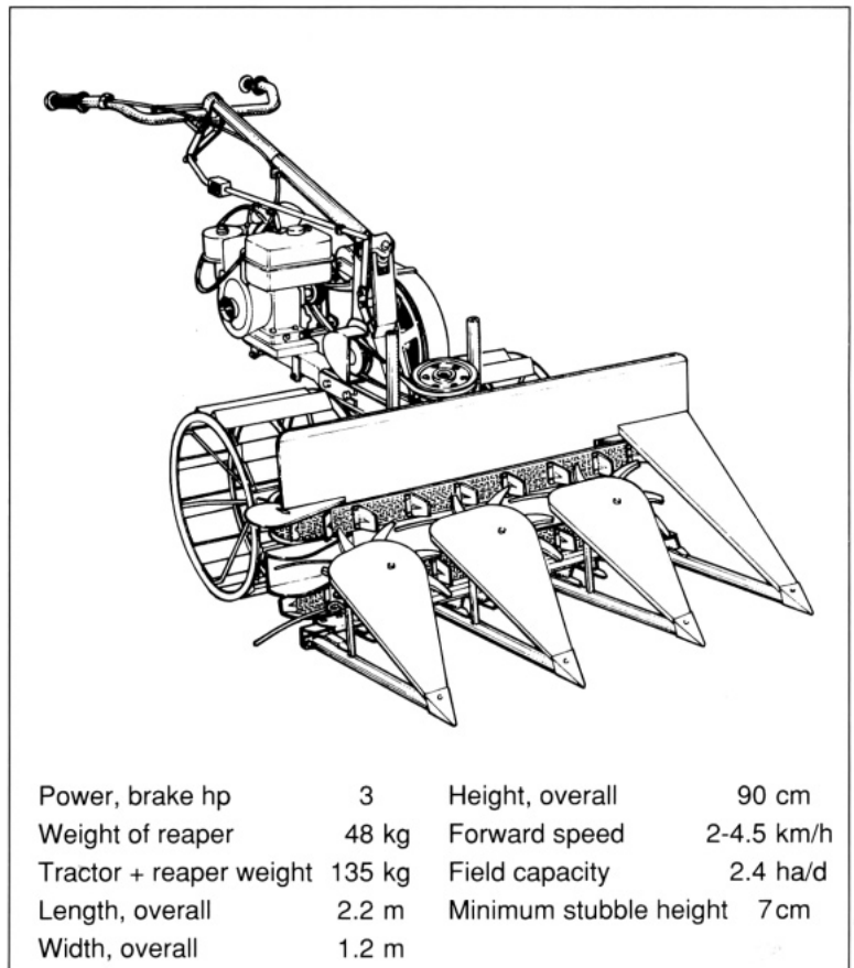
9.9. Reaper on pedestrian tractor. 2
