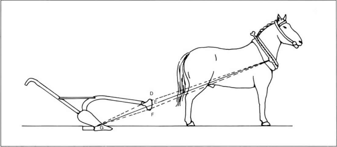
4.18. Vertical adjustment of walking plow.
