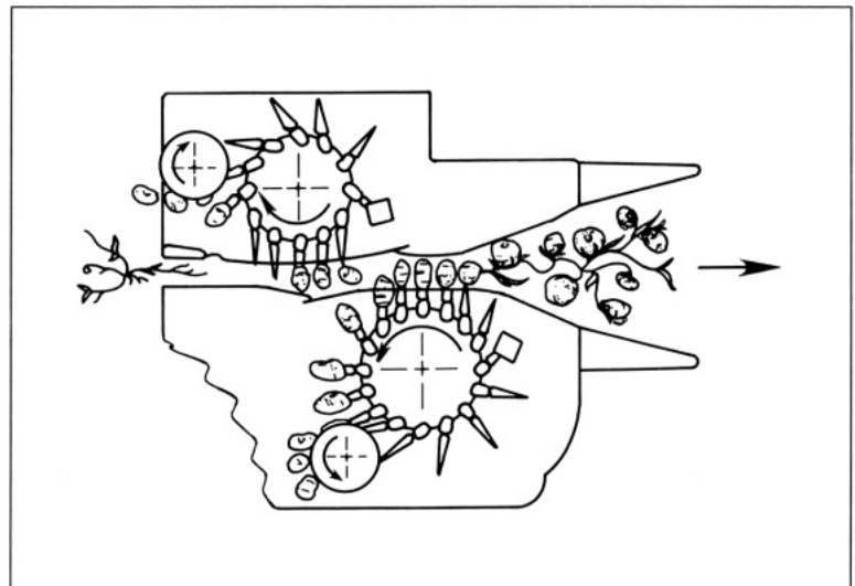
9.43. Top view of spindle picker, drum type. with tapered spindles.
