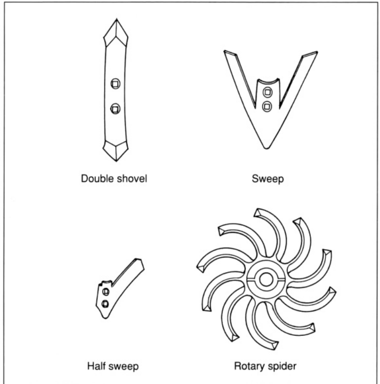
7.6. Soil-engaging elements of a typical cultivator.
