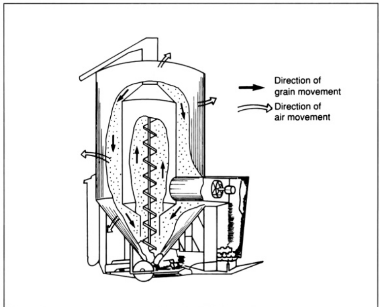
10.9. Recirculating batch dryer.
