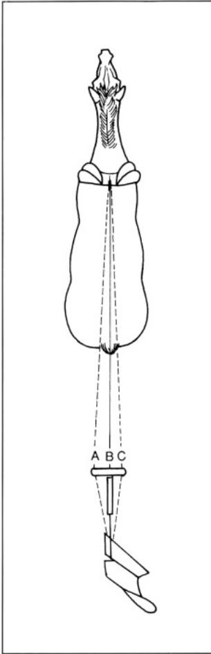
4.17. Horizontal adjustment of walking plow.
