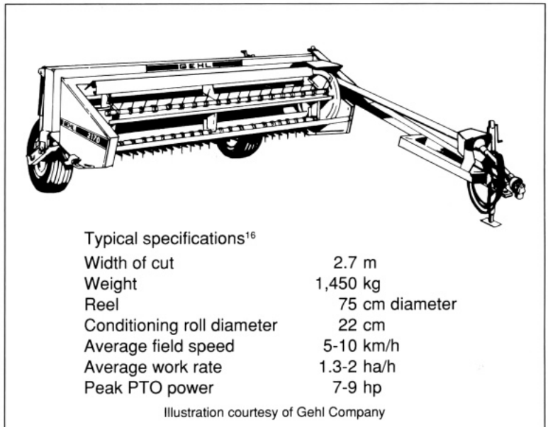
9.29. Mower-conditioner.
