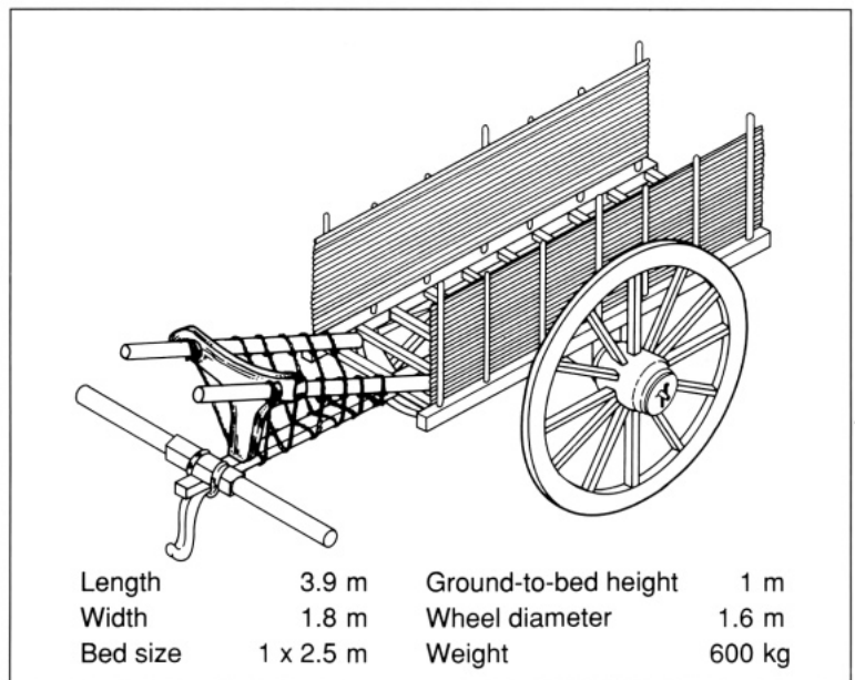
11.8. Cart drawn by a pair of bullocks (India).
