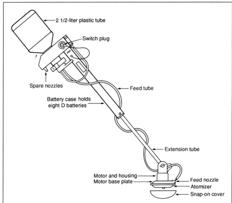
7.10. A hand-held controlled droplet application (CDA) sprayer.
