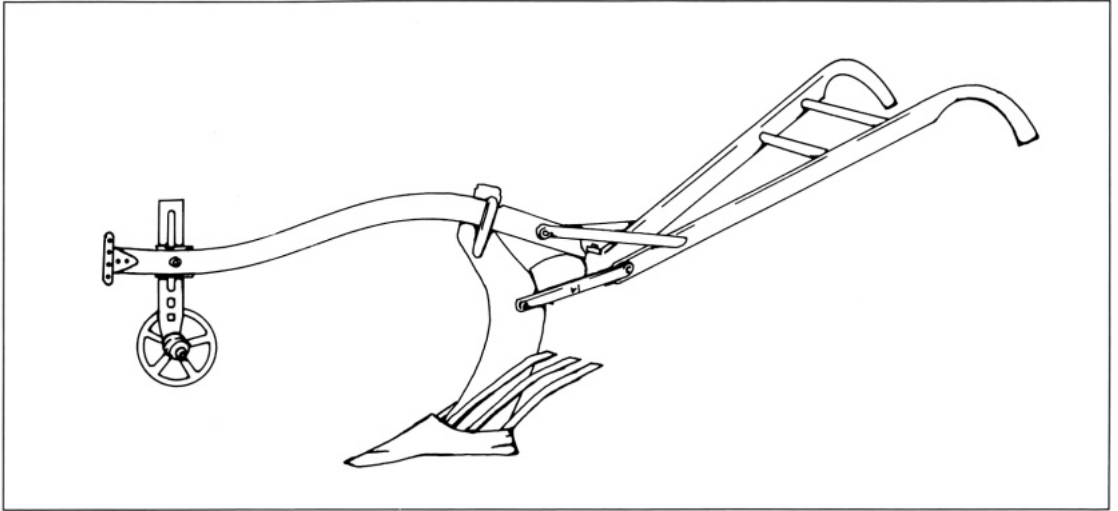
9.22. Animal-drawn potato plow.
