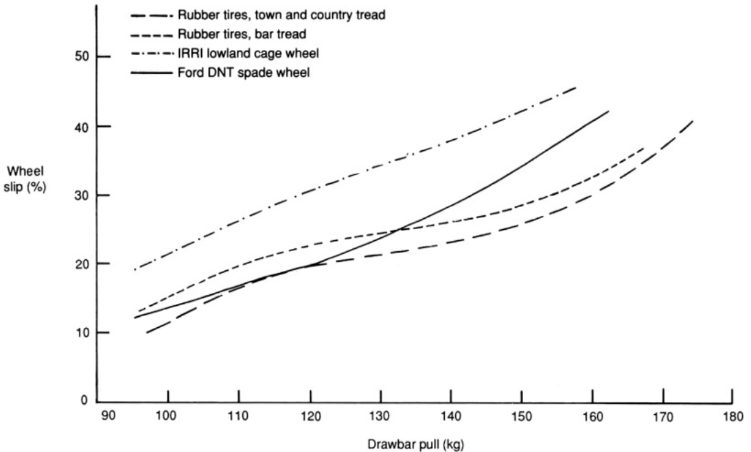
2.15. Wheel slip vs drawbar pull for a single-axle pedestrian tractor. 9
