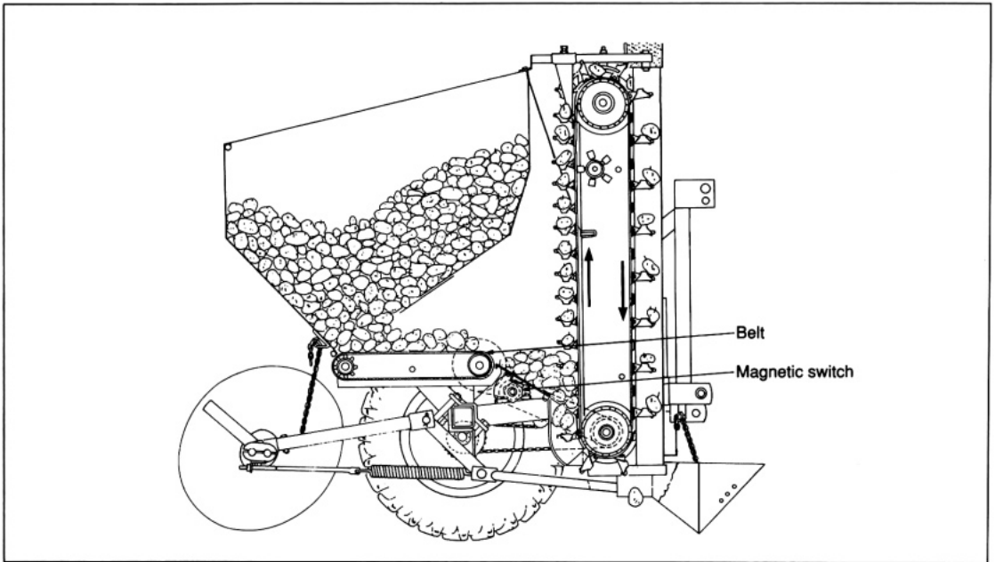
5.18. Potato planter using picker pins.
