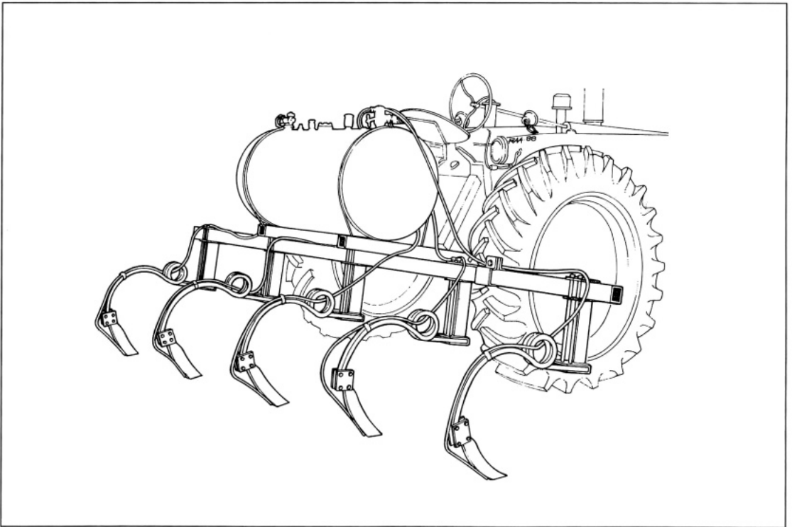
6.8. Tractor-mounted anhydrous ammonia applicator.
