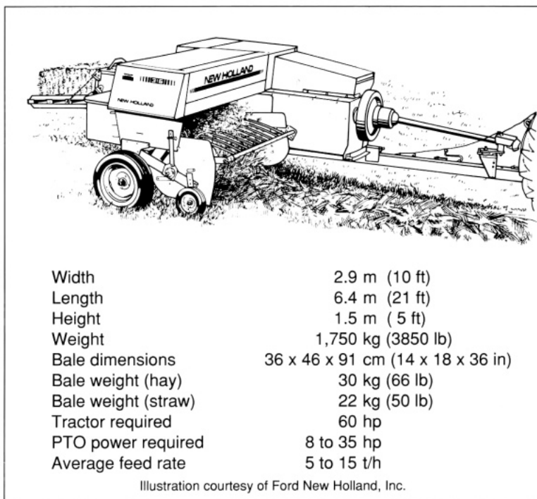
9.37. Pickup baler for making small rectangular bales. 19
