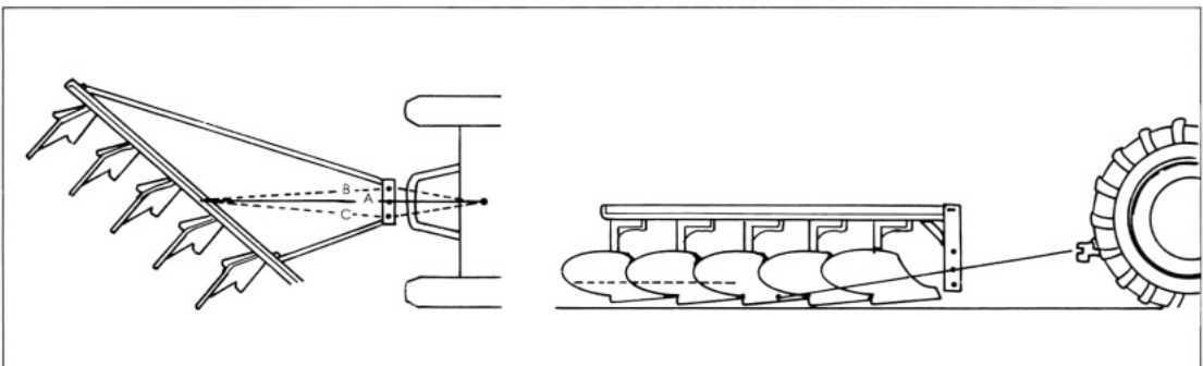
4.19. Hitching a tractor plow.
