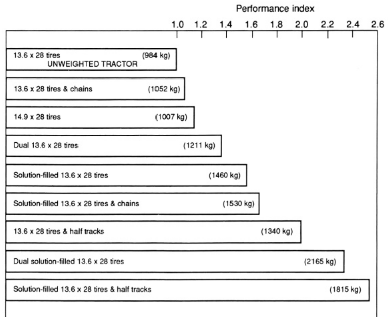
2.14. Performance of traction aids on a 45-hp 2-wheel drive farm tractor.
