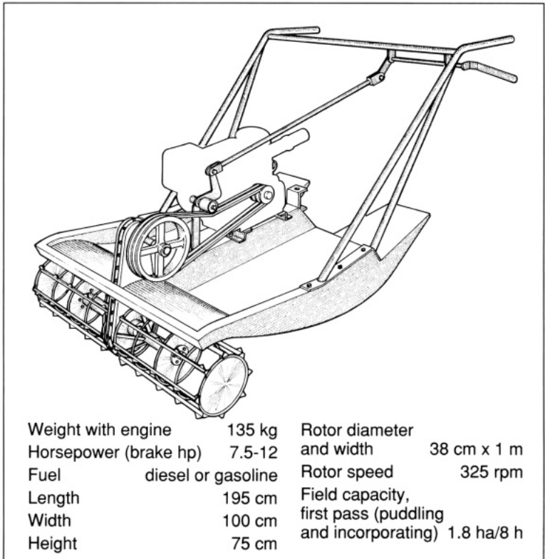
2.4. Hydrotiller, a floating rotary tiller (IRRI twin-hull design).
