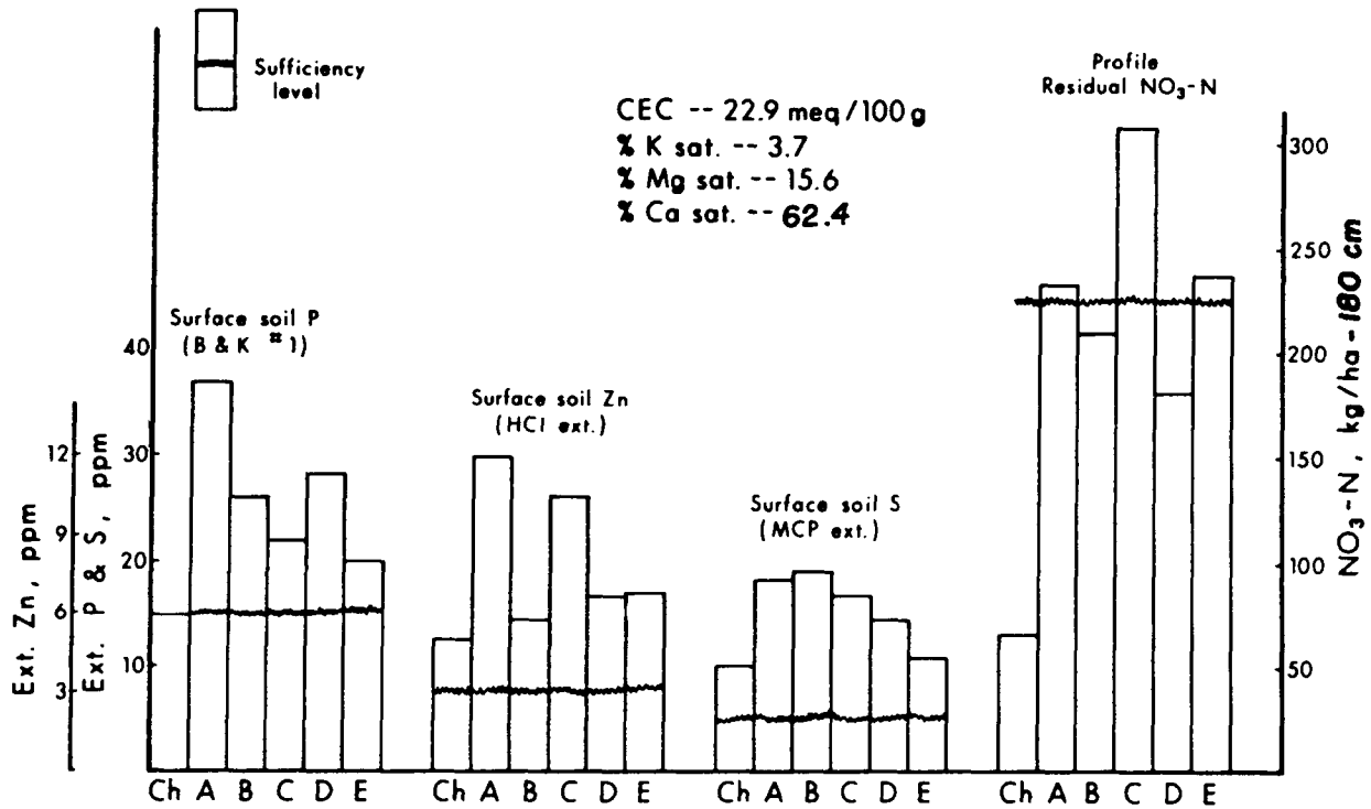
Fig. 6. Changes in nutrient status of Sharpsburg silt surface soil and profile NO 3 -N effected by the varied fertilizer programs of labs A, B, C, D and E during the 8-year study period (Cation capacity values obtained from control plots; B & K = Bray & Kurtz; ext. = extractable).
