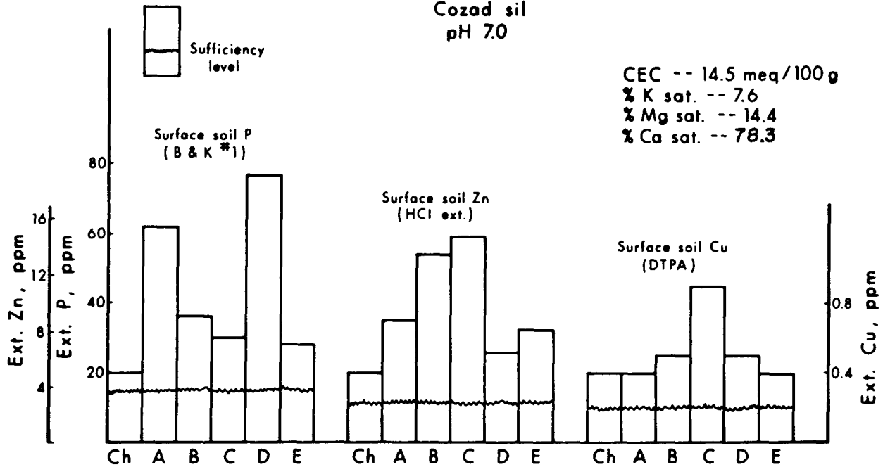
Fig. 7. Changes in nutrient status of Cozad silt surface soil effected by the varied fertilizer programs of labs A, B, C, D and E during the 7-year study period (Cation capacity values obtained from control plots; B & K = Bray & Kurtz; ext. = extractable).
