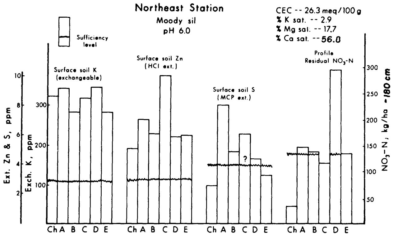
Fig. 9. Changes in nutrient status of Moody sil surface soil and profile NO 3 -N effected by the varied fertilizer programs of labs A, B, C, D and E during the 7-year period (Cation capacity values obtained from control plots. The ? on sufficiency level for S prompted by the need for profile and not just surface soil test values for S; ext. = extractable; exch. = exchangeable).
