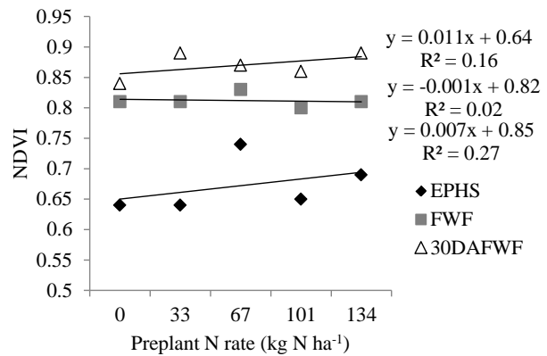
Figure 5. Effect of preplant N application on normalized difference vegetative index (NDVI) at early pinhead (EPHS), first white flower (WF), and 30 d after first white flower (30 DAFWF) cotton growth stages in 2009, Lake Carl Blackwell, OK. Note: The regression equations corresponds to the legend from top to bottom.
