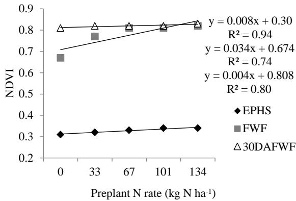
Figure 4. Effect of preplant N application at on normalized difference vegetative index (NDVI) at early pinhead (EPHS), first white flower (WF), and 30 d after first white flower (30 DAFWF) cotton growth stages in 2010, Altus, OK. Note: The regression equations corresponds to the legend from top to bottom.
