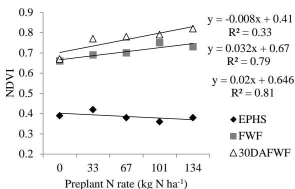
Figure 3. Effect of preplant N application on normalized difference vegetative index (NDVI) at early pinhead (EPHS), first white flower (WF), and 30 d after first white flower (30 DAFWF) cotton growth stages in 2009, Altus, OK. Note: The regression equations corresponds to the legend from top to bottom.
