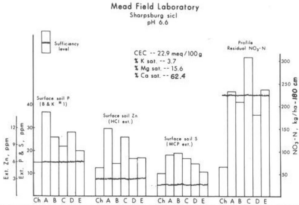
Fig. 6. Changes in nutrient status of Sharpsburg sil surface soil and profile NO 3 -N effected by the varied fertilizer programs of labs A, B, C, D and E during the 8-year study period (Cation capacity values obtained from control plots; B & K = Bray & Kurtz; ext. = extractable).
