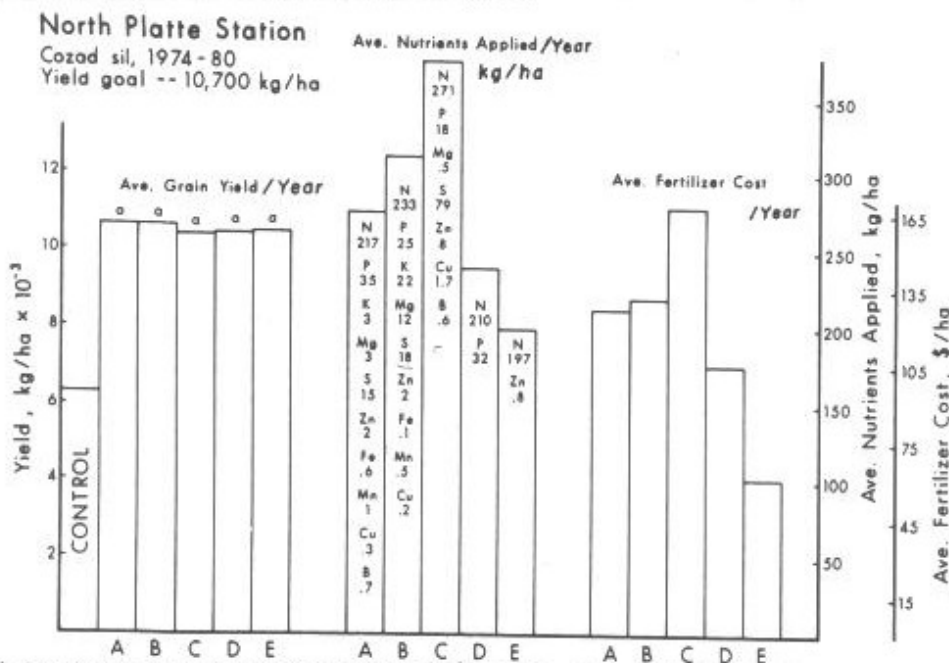
Fig. 3. Average annual grain yields, nutrients applied, and fertilizer costs for irrigated corn produced on Cozad sil, North Platte Station, with fertilizer programs recommended by labs A, B, C, D and E; 1974-80.
