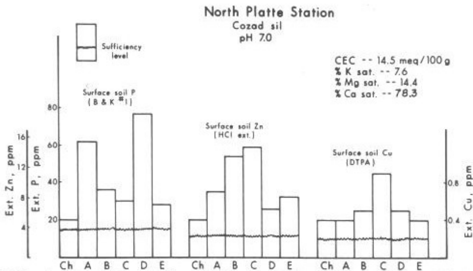
Fig. 7. Changes in nutrient status of Cozad sil surface soil effected by the varied fertilizer programs of labs A, B, C, D and E during the 7-year study period (Cation capacity values obtained from control plots; B & K = Bray & Kurtz; ext. = extractable).
