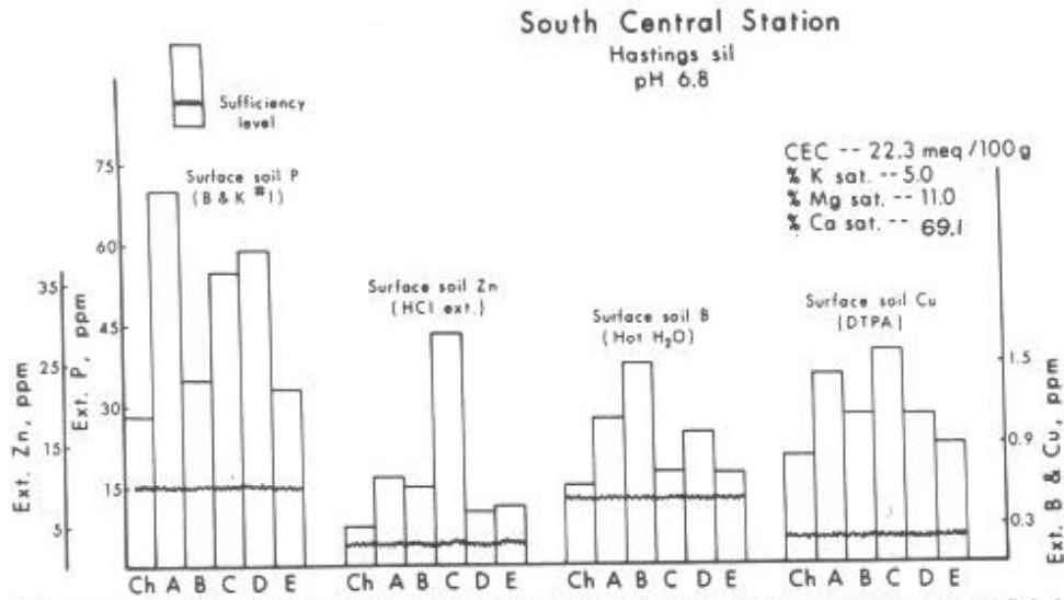
Fig. 8. Changes in nutrient status of Hastings sil surface soil effected by the varied fertilizer programs of labs A, B, C, D and E during the 6-year period (Cation capacity values obtained from control plots; B & K = Bray & Kurtz; ext. = extractable).
